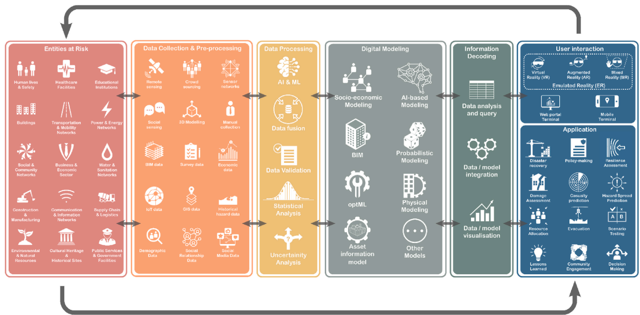
Fig. 13. Conceptualization of components of DPRMT.
